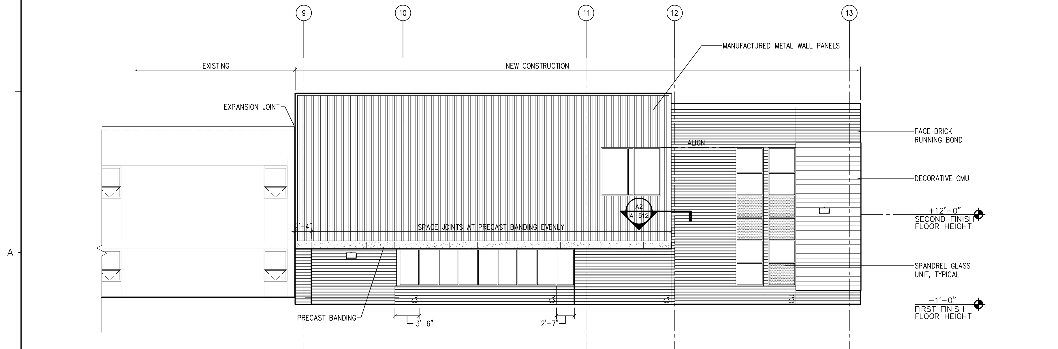
A1 SOUTH ELEVATION 1/8"=1'-0"
