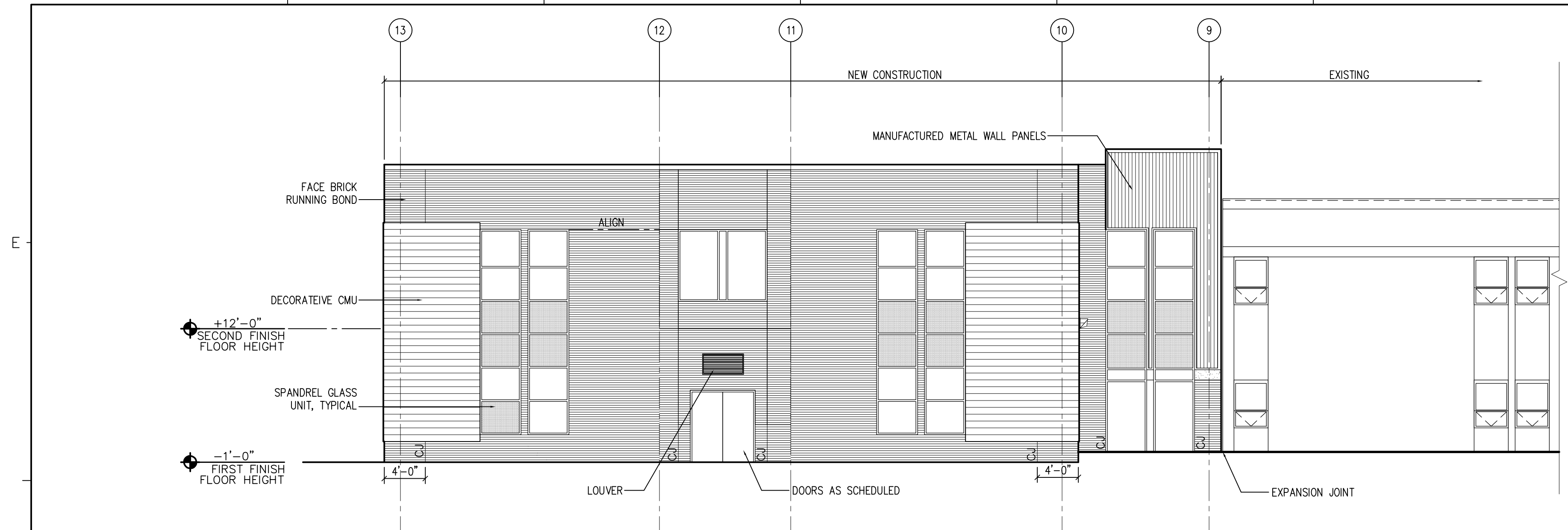
E1 NORTH ELEVATION 1/8"=1'-0"
